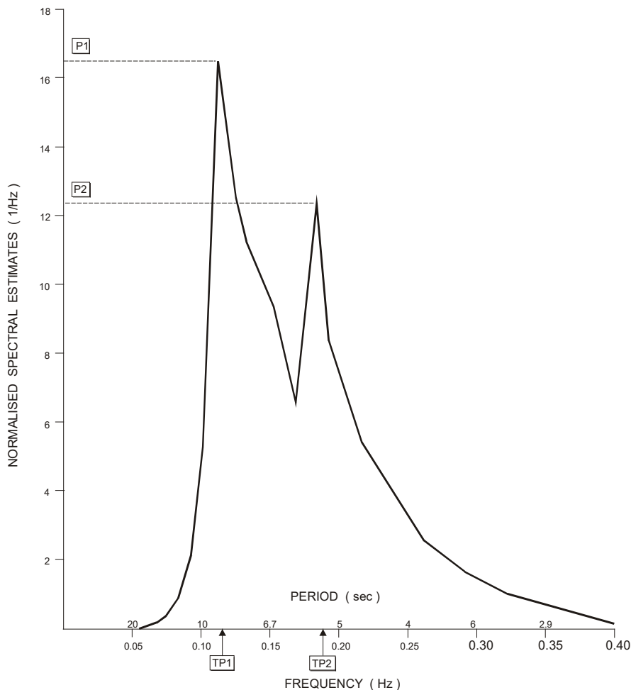
Figure 5.2 Spectral diagram
